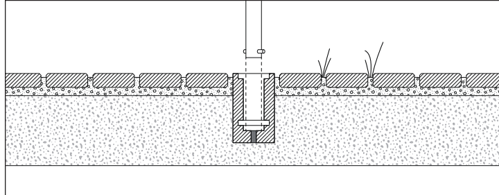
Semi-permeable soil
