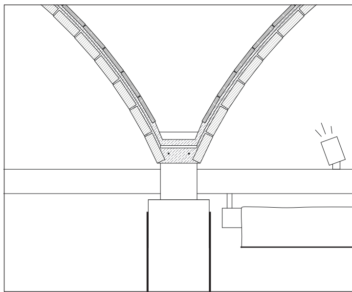
Hybrid structure: brick, pre-stressed concrete, glazed tiles
